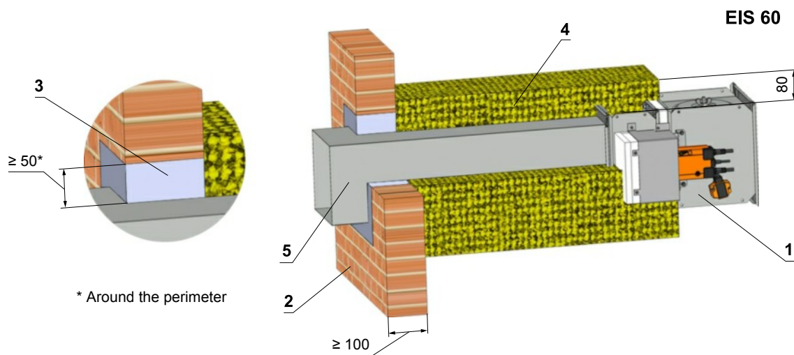
Fig. 43 Outside solid wall construction - mineral wool - mortar or gypsum
