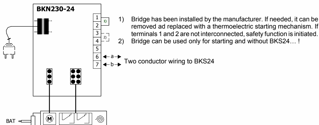
Fig. 20 Communication and supply device BKN 230-24, with act. mechanism BF 24-TN-ST (BFL 24-T-ST, BFN 24-T-ST)
