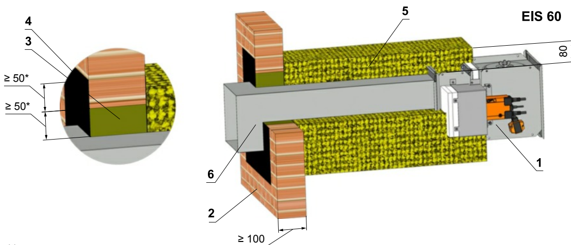
Fig. 44 Outside solid wall construction - mineral wool - stuffing box and fire protection mastic
