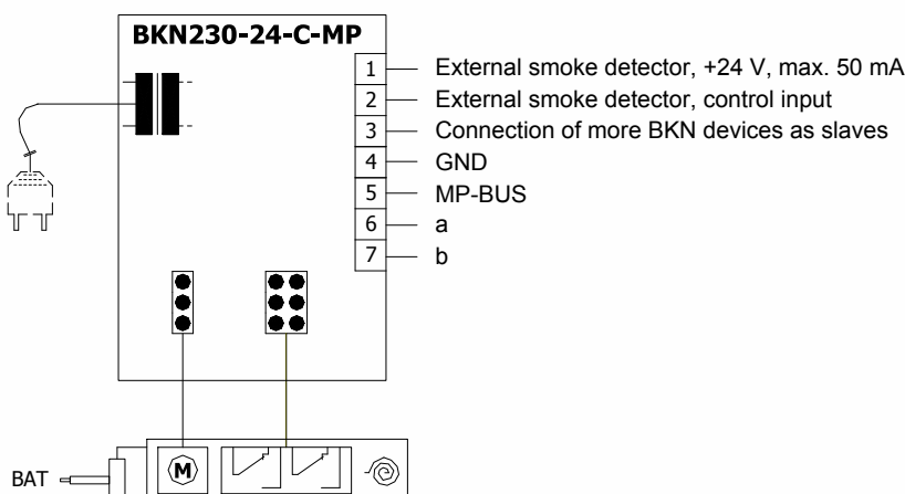
Fig. 21 Communication and supply device BKN 230-24-C-MP
