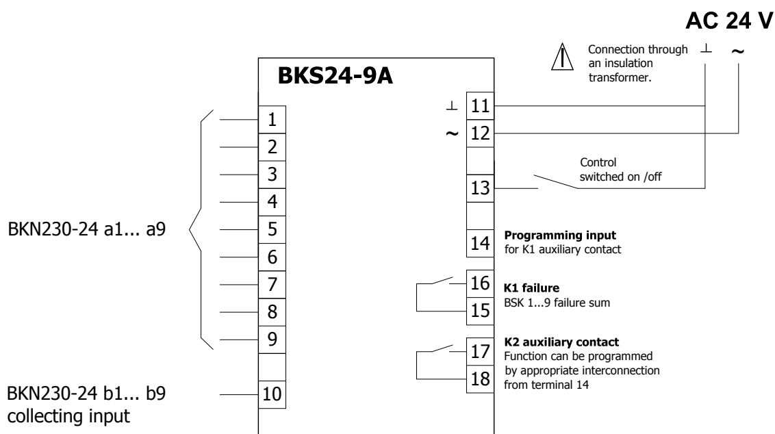
Fig. 29 Communication and control device BKS 24-9A
